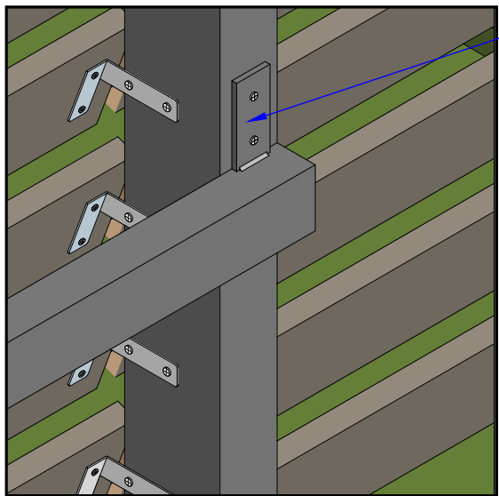
3 :: GUARD RAIL DETAIL 1 scale: NTS
